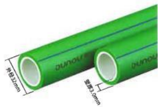
PPR双层冷水增强管PN1.25MPa
